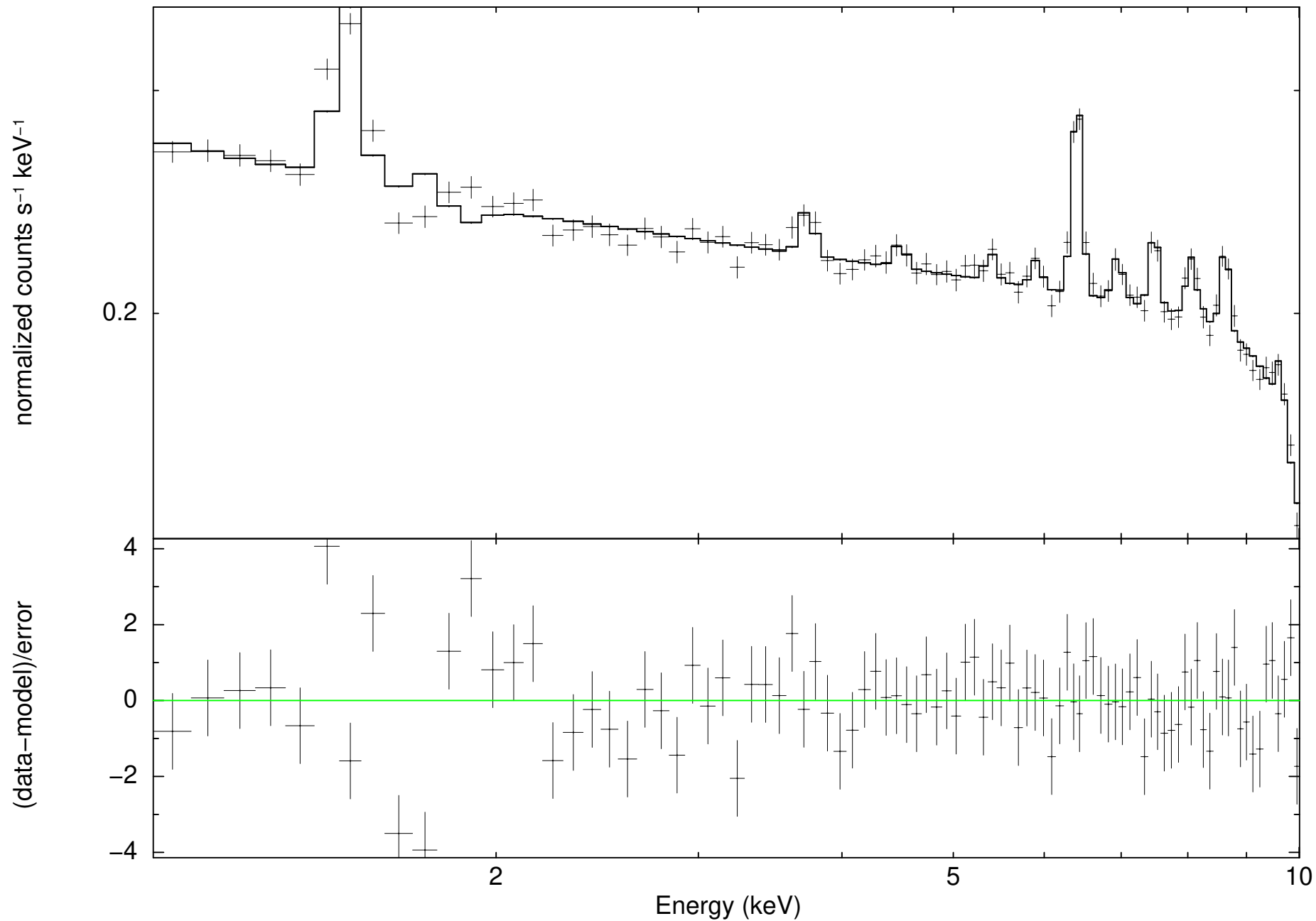
All patterns for TM7 above 1 keV (Red.Chi2=1.1306)
