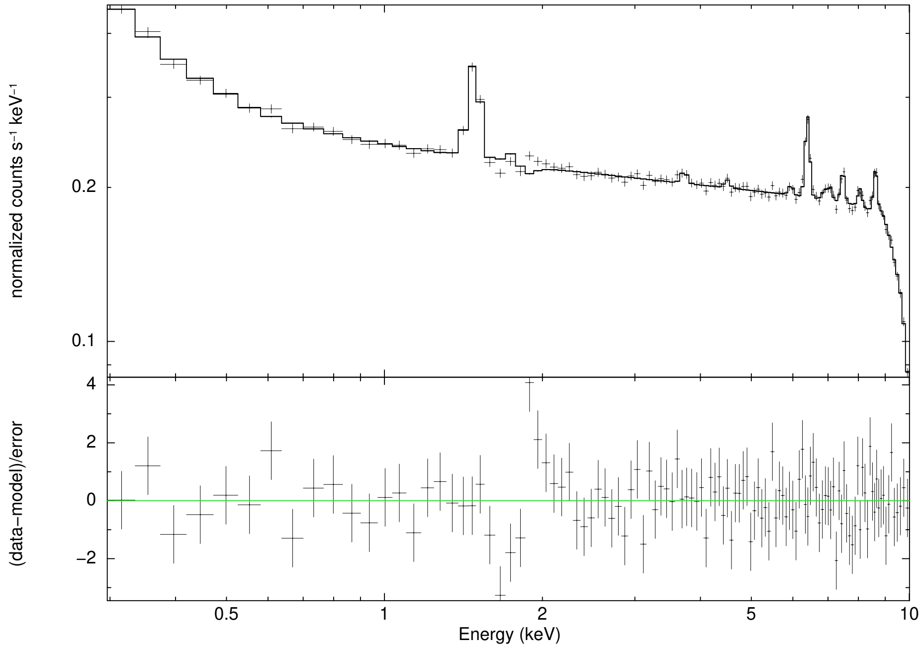
All patterns for TM4 above 0.3 keV (Red.Chi2=1.0185)
