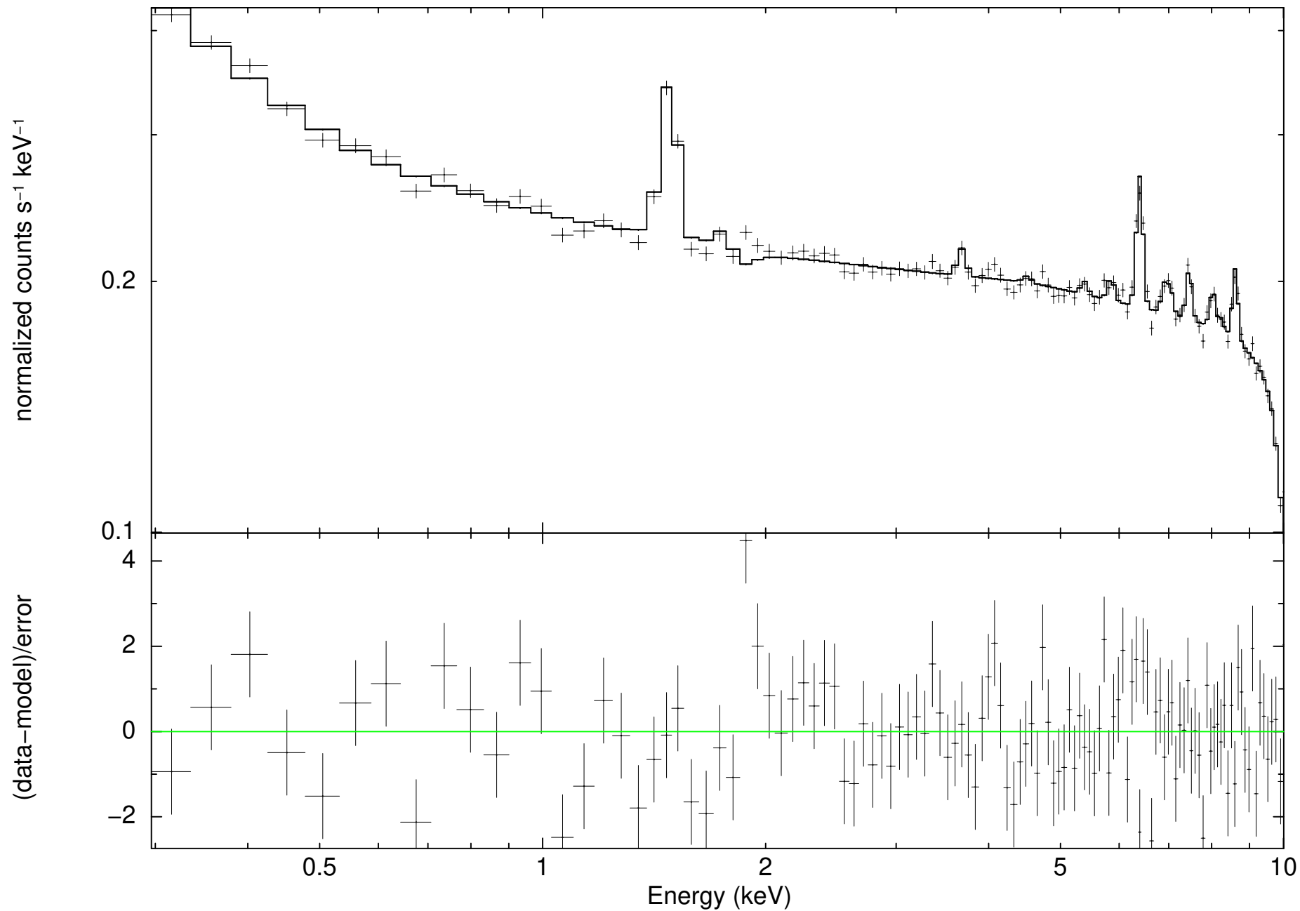
All patterns for TM3 above 0.3 keV (Red.Chi2=1.2360)
