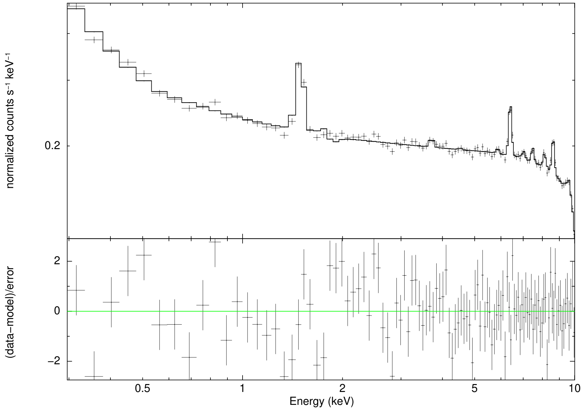
All patterns for TM2 above 0.3 keV (Red.Chi2=1.0355)
