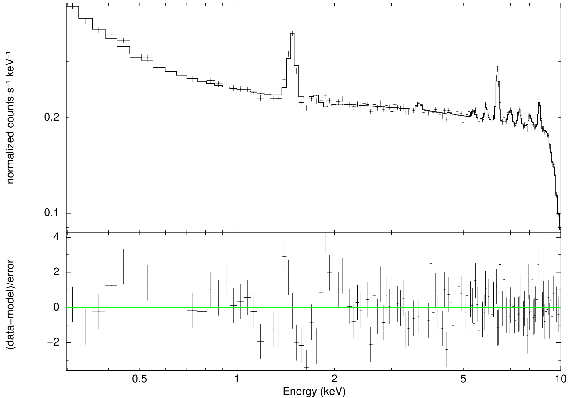
All patterns for TM1 above 0.3 keV (Red.Chi2=1.1491)
