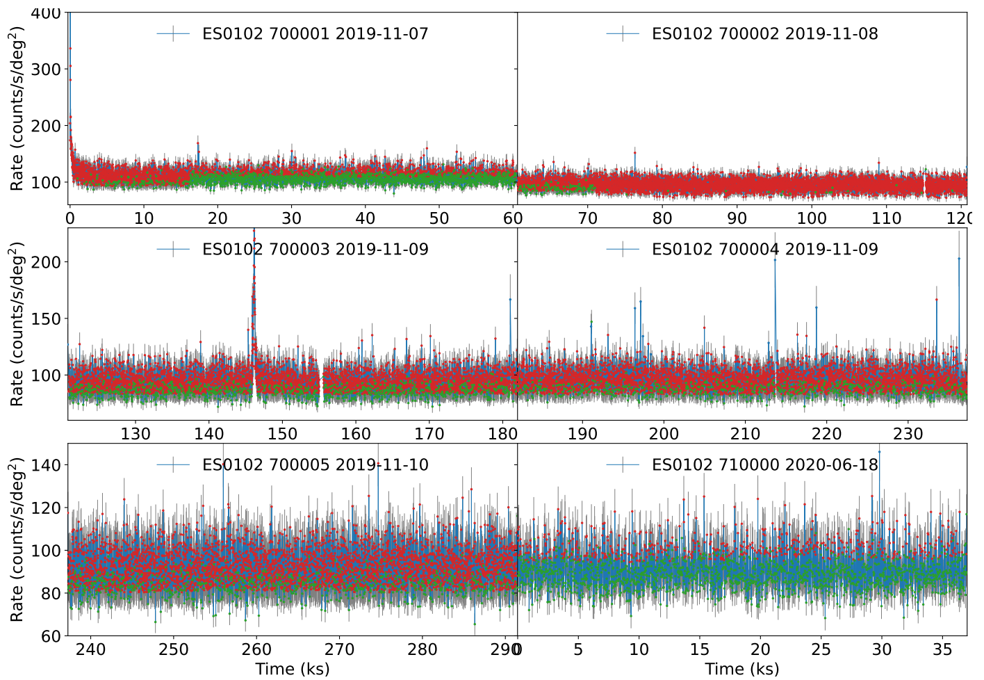
Fig. 1-a. The background light curves of each observation with 1- \sigma uncertainty. Three colors are adopted to plot the points. When the time bin has its original size of 10s, the point is plotted in red. When the bin size is 20s, i.e., resulting from merging two nearby original bins, the point is plotted in green. In other cases where more nearby original bins are merged, the point is plotted in blue.
